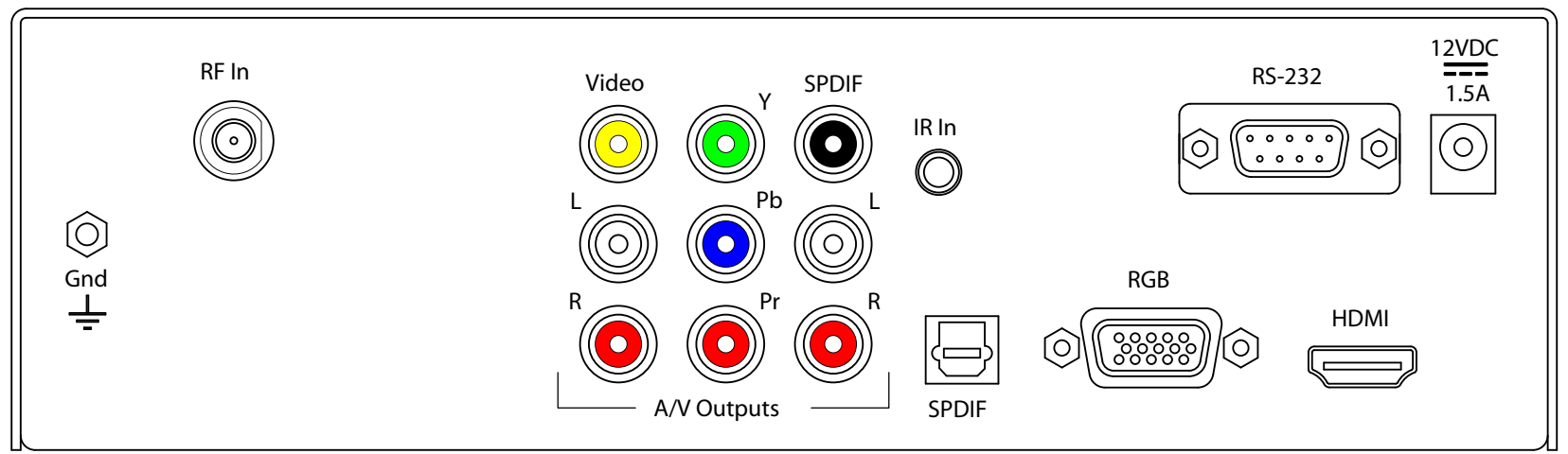
REAR VIEW
