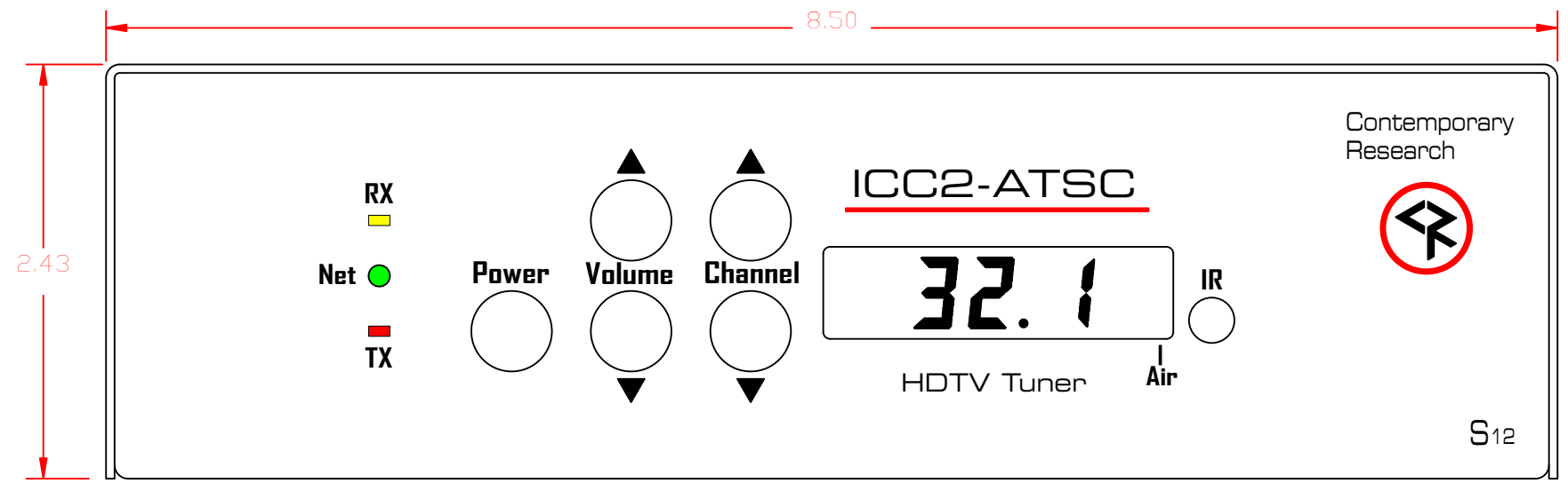
FRONT VIEW
