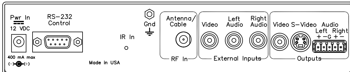
REAR VIEW
