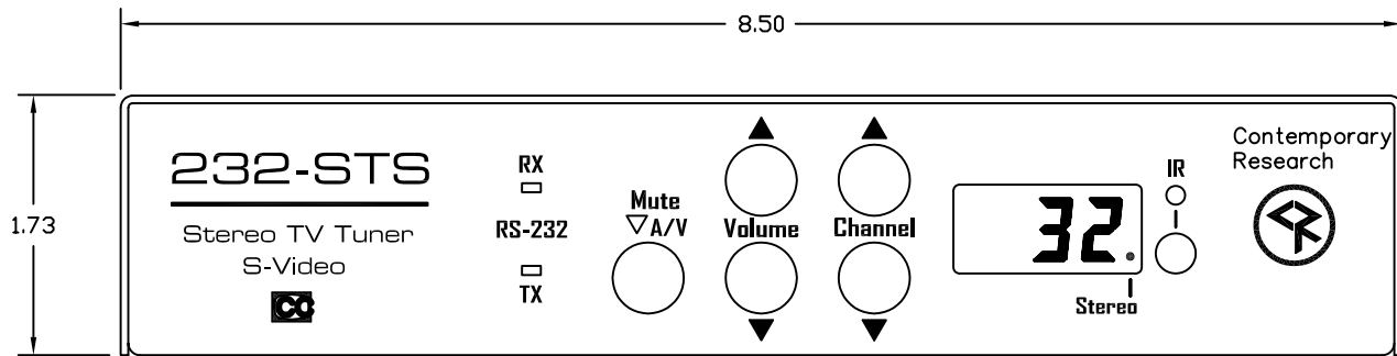
FRONT VIEW
