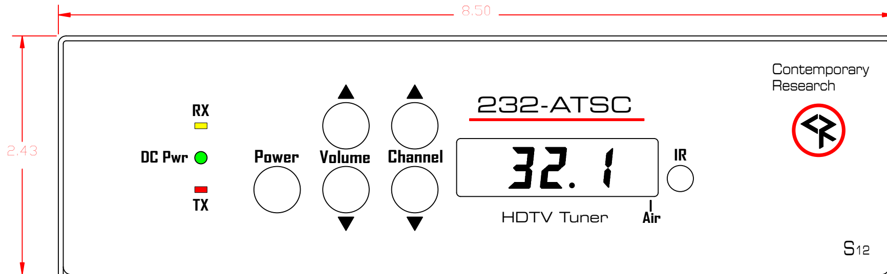
FRONT VIEW
