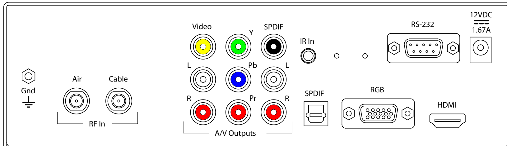
REAR VIEW
